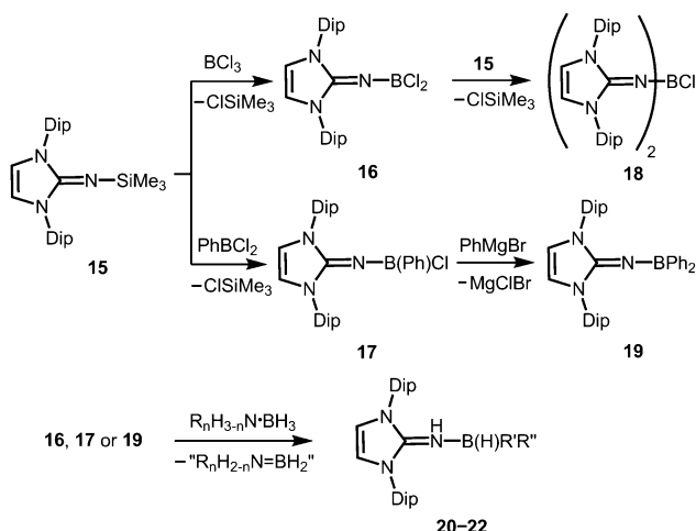
Scheme 6 Conversion of the imino trimethylsilane 15 to the imino boron chlorides 16 – 18 and the imino diphenylborane 19 . Formation of the imine–borane adducts via abstraction of dihydrogen from amine–borane adducts.
