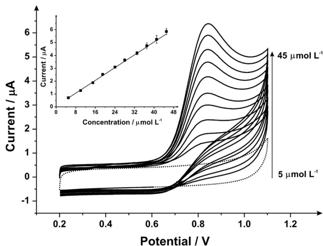
Fig. 7 Cyclic voltammograms obtained from additions of sodium nitrite ( 5\text{--}45\text{ }\mu\text{mol L}^{-1} ) into pH 7 PB using a 1 minute mechanically activated/polished SPE with diamond slurry using the same SPE throughout the experimentation (scan rate: 100\text{ mV s}^{-1} vs. SCE); the dotted line represents the blank (no sodium nitrite) response. Inset: analysis of the voltammetric peak heights as a function of concentration.
