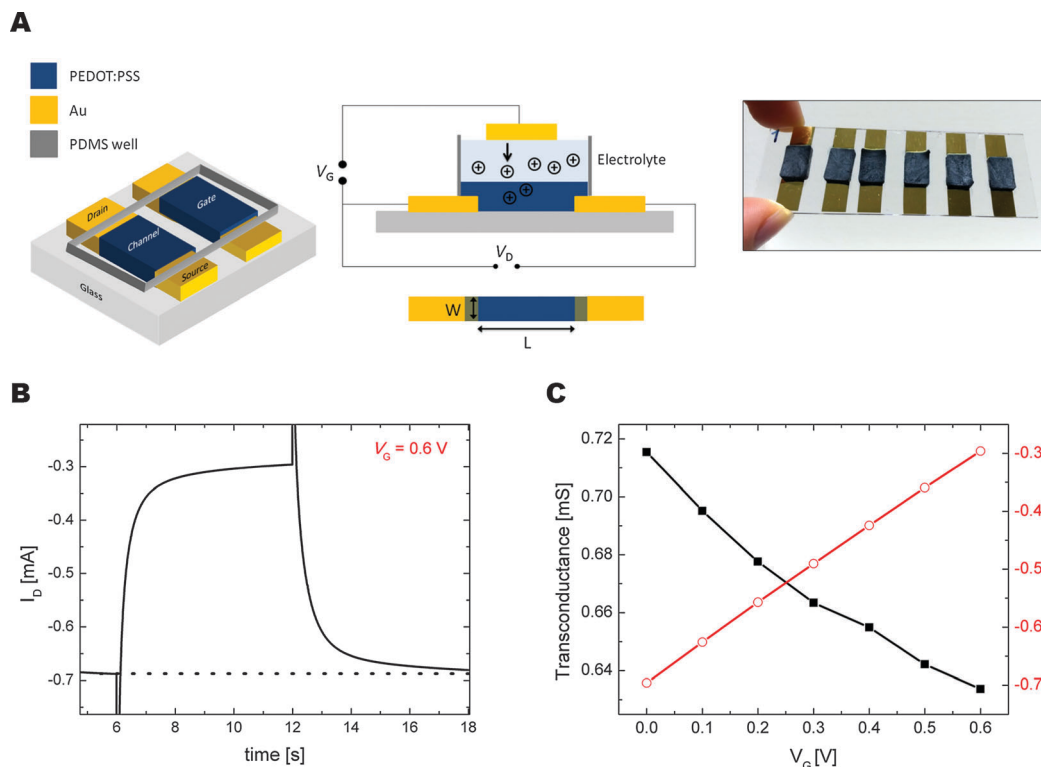
Fig. 2 (A) 3D, cross sectional, and top view schematics of the OECT structure where W = 6 mm and L = 6 mm (figure not to scale). The photograph at right shows typical OECTs. The conductivity of the PEDOT:PSS scaffold interfacing the source and drain electrodes decreases by the injection of cations from the electrolyte, triggered by an applied bias through the second scaffold which acts as the gate electrode. (B) Transient characteristics of a transistor ( W = 6 mm, L = 6 mm, d = 2 mm) prepared from a porous scaffold. The length of the pulse at the gate electrode ( V_G = 0.6 V) was 6 s. V_D was constant at -0.6 V. (C) Transfer characteristics of an OECT comprised of a porous scaffold, and corresponding transconductance values at V_D = -0.6 V.
