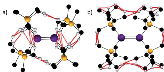
Fig. 3 H–H and C–H distances below the sum of the van der Waals radii (2.4 and 2.9 Å respectively indicated in red) for [Sn{CH(SiMe 3 ) 2 } 2 ] 2 (a) and [Sn{SiMe t Bu 2 } 2 ] 2 (b).
