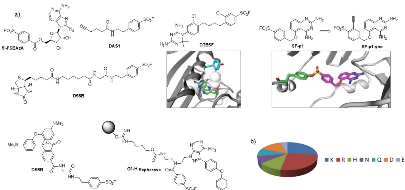
Fig. 7 (a) SF probes that react with tyrosine: 5'-FSBAzA; DAS1; DS6B; DS6R; G1-H sepharose resin; DTBSF and complex of bioplerin (green) in chicken liver DHFR (PDB 1DR1) showing proximity of Tyr31 (cyan) which reacts with DTBSF; SF-p1 and clickable probe SF-p1-yne (and crystal structure of SF-p1 with DcpS, PDB 4QDV). (b) Pie chart showing the distribution of amino acid residues proximal to known SF-reactive tyrosines as determined by analyzing crystal structures in the PDB. 90
