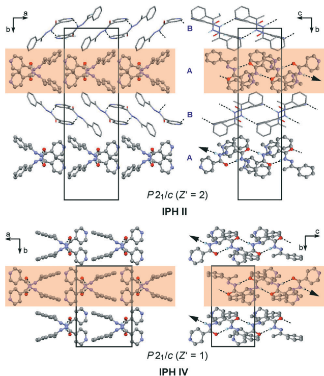
Fig. 10 Two-dimensional similar packing of molecules, based on Y-type N-H...O=C-bonded chains, in the IPH polymorphs II (molecule type A only) and IV. Each structure is viewed parallel (left) and perpendicular (right) to the direction of translation of its H-bonded chains (indicated by an arrow), with one instance of the SC Y1 highlighted (orange). All hydrogen atoms, except for those involved in hydrogen bonding, are omitted for clarity.
