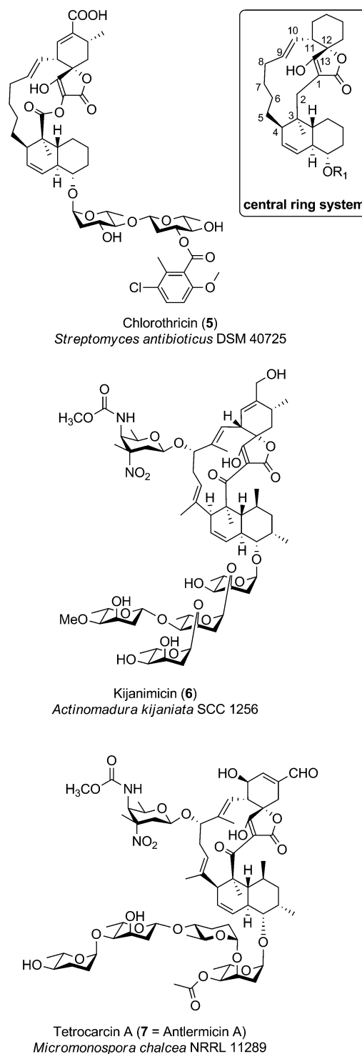
Fig. 6 Medium-sized spiroketones. The central ring system, present in the CHL/KIJ/TCA (chlorothricin/kijanimicin/tetrocarcin A) – family comprises a central 13-membered macrocycle (carbon numbering see upper right).
