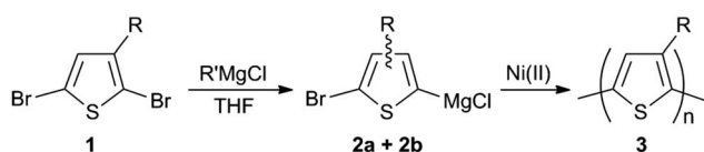
Scheme 1 Two-step synthesis of poly(3-alkylthiophenes) via Grignard metalation and polymerisation.
