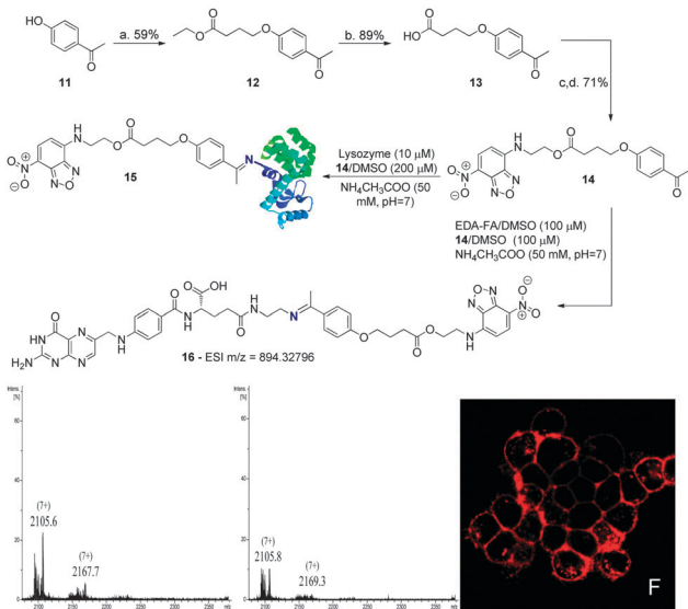
Scheme 5 (a) Ethyl 4-bromobutyrate, K_2CO_3 , NaI, acetone, reflux, 20 h; (b) TFA, H_2O , 90\text{ }^\circ C , 3 h; (c) DMAP, EDC; DCM, 0\text{ }^\circ C , 1 h; (d). NBDNH(CH _2 ) _2 OH, DCM, rt, 5 h. UV spectrum: see ESI† for compound 14 . Reaction of lysozyme ( 10\text{ }\mu M ) with 14 ( 200\text{ }\mu M ) in acetate buffer ( 50\text{ mM} , pH 7) at room temperature. Zoom of the (7+) charge state of the ESI-FTICR-MS spectra after 30 min and 2 h of reaction. Image F shows NCI-H460 treated with compound 16 . Incubation and imaging conditions are likewise described in Scheme 3.
