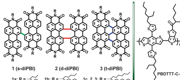
Fig. 1 The chemical structures of bay-linked PBIs (diPBIs, 1–3 ) and donor polymer (PBDDTTT-C-T) used in this study.
