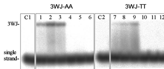
Fig. 10 Autoradiograms of the gels run at room temperature. Lane C1: control containing the three strands, S1-AA, S2 and S3. Lanes 1–3: S1-AA, S2 and S3 mixed with \Delta_{\text{Fe}}\text{-}[\text{Fe}_2\text{L}^{1a}_3]\text{Cl}_4 at 0.5 : 1, 1 : 1 and 2 : 1 (flexicate : 3WJ) ratios, respectively. Lanes 4–6: S1-AA, S2 and S3 mixed with \Delta_{\text{Fe}}\text{-}[\text{Fe}_2\text{L}^{1a}_3]\text{Cl}_4 at 0.5 : 1, 1 : 1 and 2 : 1 (flexicate : 3WJ) ratios, respectively. Lane C2: control containing the three strands, S1-TT, S2 and S3. Lanes 7–9: S1-TT, S2 and S3 mixed with \Delta_{\text{Fe}}\text{-}[\text{Fe}_2\text{L}^{1a}_3]\text{Cl}_4 at 0.5 : 1, 1 : 1 and 2 : 1 (flexicate : 3WJ) ratios, respectively. Lanes 10–12: S1-TT, S2 and S3 mixed with \Delta_{\text{Fe}}\text{-}[\text{Fe}_2\text{L}^{1a}_3]\text{Cl}_4 at 0.5 : 1, 1 : 1 and 2 : 1 (flexicate : 3WJ) ratios, respectively.
