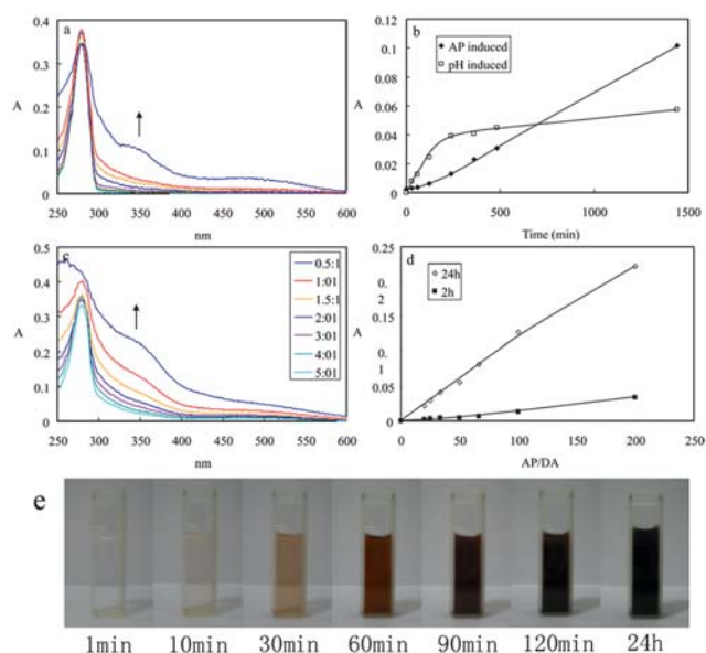
Fig. 1 (a) UV-vis spectra of DA during the AP-mediated oxidation reaction. (b) Absorption intensity at 350 nm of DA by both oxidant-induced and pH-induced. (c) UV-vis spectra of DA after 24 h running time by mixed with different amount of AP. (d) Absorption intensity at 350 nm of DA after 2 h and 24 h running time when mixed with different amounts of AP. (e) Colour change of DA with the running time.
