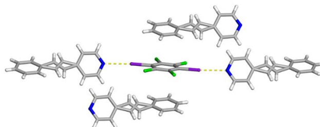
Figure 6. X-ray structure of Form II illustrating the I...N halogen bonds as well as the heterogeneous \pi - \pi stacking arrangement of \text{C}_6\text{I}_2\text{Cl}_4 . The I...N halogen bonds are shown with yellow dashed lines. The disorder observed in \text{C}_6\text{I}_2\text{Cl}_4 was removed for clarity.
