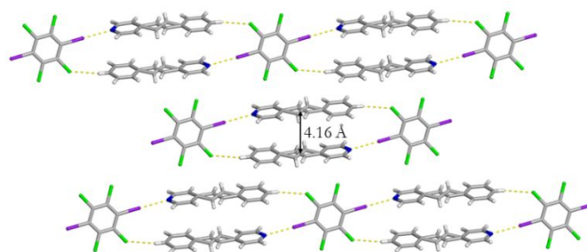
Figure 2. X-ray structure of Form I illustrating the anti -orientation within the one-dimensional chain. The I...N halogen bonds and C-H...Cl contacts are shown with yellow dashed lines.
