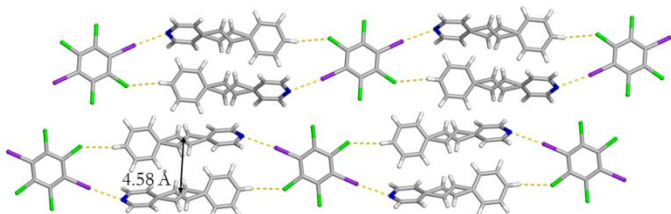
Figure 5. X-ray structure of Form II illustrating the anti -orientation within the one-dimensional chain. The I...N halogen bonds and C-H...Cl contacts are shown with yellow dashed lines. The disorder observed in \text{C}_6\text{I}_2\text{Cl}_4 was removed for clarity.
