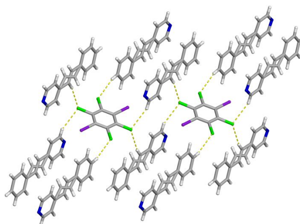
Figure 3. X-ray structure of Form I illustrating all of the different types of C-H...Cl contacts. The C-H...Cl contacts are shown with yellow dashed lines.
