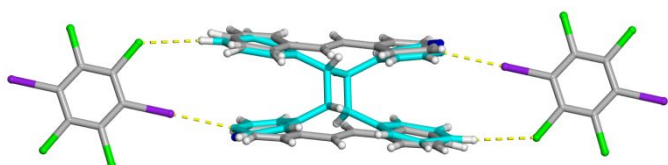
Figure 4. X-ray structure of the partially photoreacted co-crystal of Form I forming the ht-PP shown in turquoise. The I...N halogen bonds and C-H...Cl contacts are shown with yellow dashed lines.
