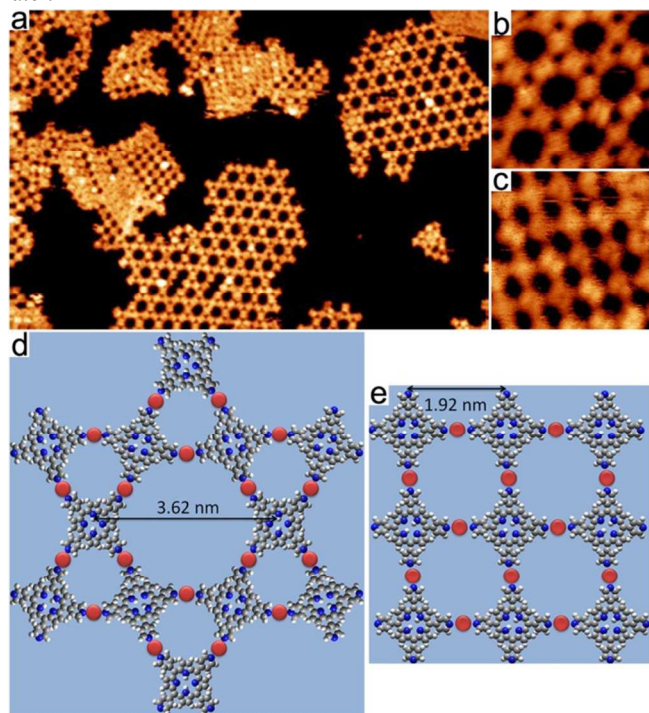
Fig. 3 (a) STM topograph showing 3 and Pb form close-packed islands, Kagome and rhombus porous networks ( 90 \times 60 nm 2 ). (b) and (c) High-resolution images of the Kagome and rhombus networks ( 12 \times 12 nm 2 ). (d) and (e) Structural models of the Kagome and rhombus networks.
