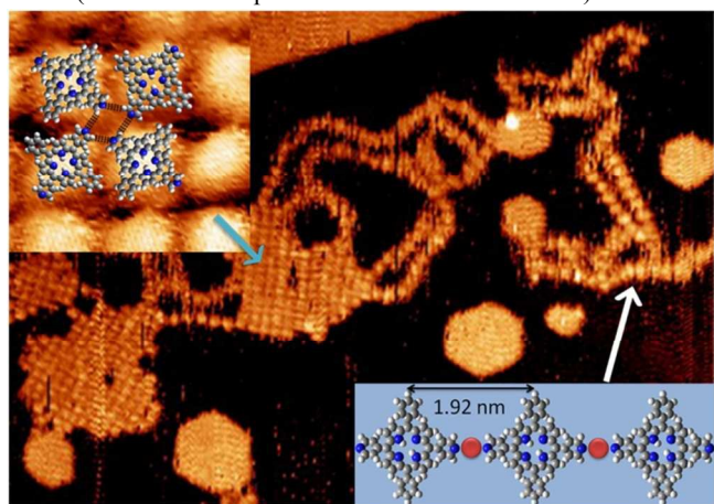
Fig. 1 (a) An overview STM topograph showing 1 and Pb form SR chains ( 100 \times 70 \text{ nm}^2 ). Up-left inset: magnified view of a closely-packed network ( 4 \times 4 \text{ nm}^2 ) with a tentative model overlaid. The dashed lines indicate hydrogen bonds. Bottom-right inset: Structural model of the SR chain. Color code: C, gray; N, blue; H, white; Pb, red.
