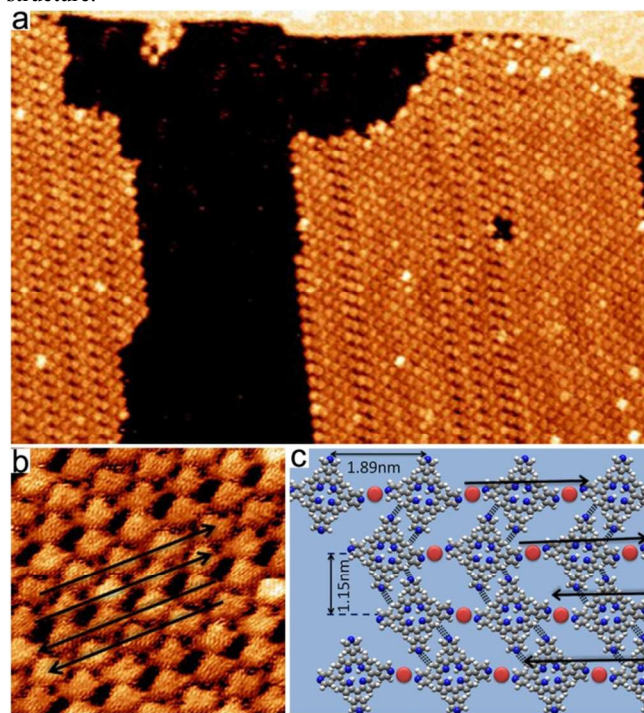
Fig. 4 (a) An overview STM topograph of MR structure ( 90 \times 60 nm 2 ). (b) High-resolution image ( 10 nm \times 10 nm 2 ). The arrows highlight the rows. (c) Structural model of the MR structure. The dashed lines indicate hydrogen bonds. The arrow direction indicates the azimuth rotation of the molecules in that row.
