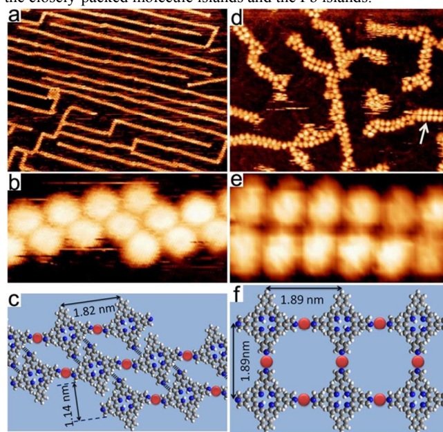
Fig. 2 (a) and (d) STM topographs showing DR chains and the ladder structures formed out of 2 and Pb ( 113 \times 151 \text{ nm}^2 and 54 \times 72 \text{ nm}^2 ), respectively. (b) and (e) High-resolution images of a DR chain and a ladder structure ( 5 \times 10 \text{ nm}^2 ). (c) and (f) Structural models of the DR chain and the ladder structure, respectively. The dashed lines indicate hydrogen bonds.
