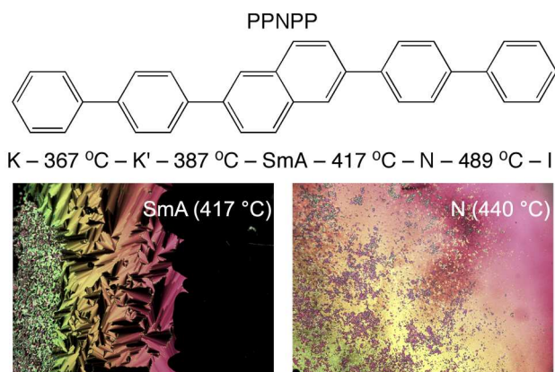
Fig. 2. Molecular structure and phase map of PPNPP (measured on first heating by DSC; heating rate 20 °C/min). The microphotographs show the focal conic texture of the SmA phase at 417 °C and the high temperature nematic phase at 440 °C. The black area in the former picture is an air bubble due to the material rapid sublimation.
