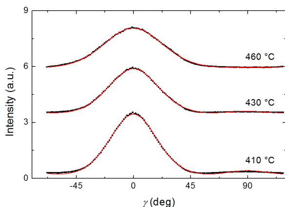
Fig. 7. Azimuthal intensity profile of the XRD wide-angle feature at three different temperatures (black dots) and the best fit curves (red lines). The order parameter, \langle P_2 \rangle , calculated from the fits is: 0.67 at 410 °C; 0.62 at 430 °C; 0.49 at 460 °C.
