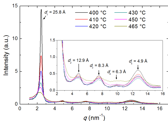
Fig. 4. Intensity profiles of the XRD pattern along the meridional direction at different temperatures (the inset is a zoom on the lower peaks); arrows indicate the d -spacing corresponding to each peak at 400 °C.
