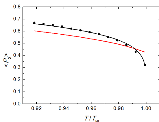
Fig. 8. Orientational order parameter as a function of the reduced temperature: measured values (black dots), fitting by Haller equation (Eq. 5, black line), and theoretical prediction from M-S theory (red line). For the last we have used the approximated expression \langle P_2 \rangle = (1 - 0.98T/T_{NI})^{0.22} , assuming a temperature independent molar volume. 20
