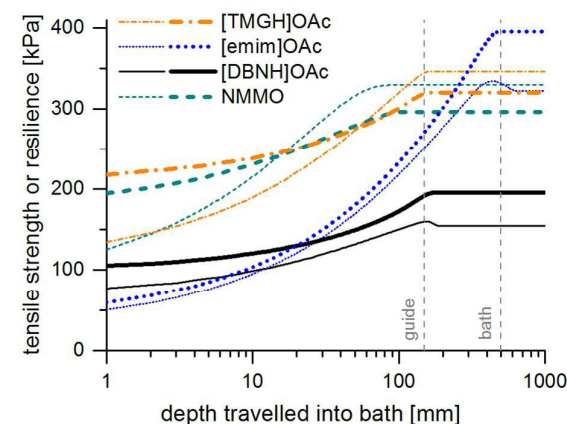
Fig. 4 Simulated minimum incipient filament strengths (thin lines) and resiliences (thick lines) at v_e = 0.05 \text{ ml/min} at D_R = 10 \text{ in kPa} as a function of distance travelled in a water bath
