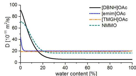
Fig. 7 Functions of the IL diffusion constants vs. water content that fit the data in Fig. 4
