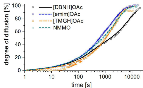
Fig. 6 Progress of diffusion of IL from a cast disc of dope into a stirred volume of water at 15 °C, observed by measuring the conductivity of the water.
