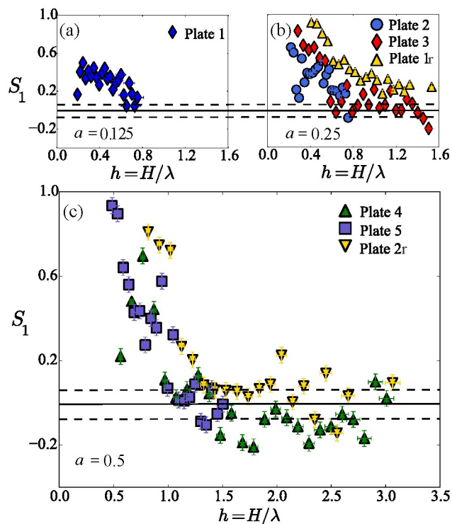
Fig. 9 The orientational order parameter S_1 (Eq. 1) describes how well-aligned individual peds (continuous regions, entirely bounded by cracks) are with the orientation of their substrate. Results are given for wave plates with dimensionless amplitudes (a) a = 0.125 , (b) a = 0.25 and (c) a = 0.5 . The solid and dashed lines represent the mean and standard deviation of measurements of S_1 on flat plates.
