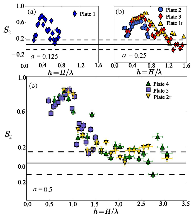
Fig. 11 The crack alignment order parameter S_2 (Eq. 2) measures the relative alignment of the cracks with the substrate, and takes large values for networks with cracks that are parallel or perpendicular to the underlying relief. Shown are the results for (a) a = 0.125 , (b) a = 0.25 , and (c) a = 0.5 . The solid and dashed lines represent the mean and standard deviation of S_2 for the flat plate.
