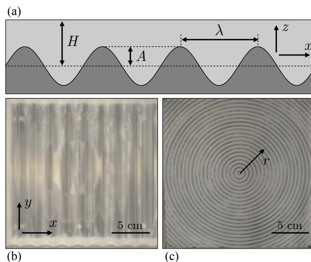
Fig. 2 Sketch of the drying experiment, where (a) a clay slurry of average initial thickness H dries over a sinusoidally varying substrate, of amplitude A and wavelength \lambda . Both (b) linear and (c) radial wave plates were used as substrates.
