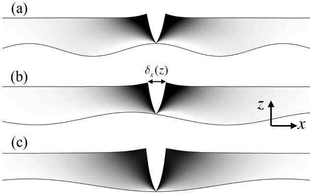
Fig. 12 Numerical solution of a channel crack opening (a) over a peak, (b) between a trough and peak and (c) over a trough of the substrate. The three cases correspond to A = 0.2 , and \lambda = 4, 6 , and 8 , respectively. The deformations caused by the cracks are exaggerated, so as to be visible, while the greyscale shows how much of the pre-crack stress \sigma_{xx}^* is released by the crack – with black shown where all the stress is released, and white where the crack does not affect the stress at all. The location of the displayed cracks are those that maximise G(\psi) for the different geometries.
