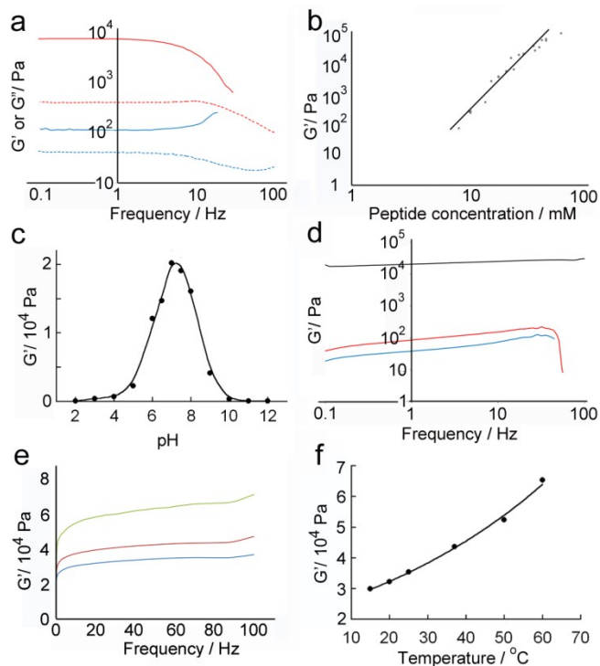
Figure 6: Quantitative analysis of hydrogel mechanical properties using oscillatory shear rheometry. a) Frequency sweeps of standard hydrogel samples containing total peptide concentrations of 10 mM [ G' (—), G'' (---)] and 5 mM [ G' (—), G'' (---)]. b) Plot showing the relationship between \log(G') and \log(\text{peptide concentration}) in hydrogels (linear curve fit to guide the eye). c) Plot of G' versus hydrogel pH obtained under strain-sweep conditions, demonstrating that maximum stiffness is attained at around pH 7.2 (curve fit to guide the eye). d) Frequency sweeps of standard hydrogel samples formed at pH 3 (—), 7 (—), and 11 (—). e) Frequency sweeps of standard hydrogel samples separately formed at 20 °C (—), 37 °C (—) and 60 °C (—). f) Plot of G' versus hydrogel temperature of a sealed sample, showing a non-linear relationship (curve fit to guide the eye).
