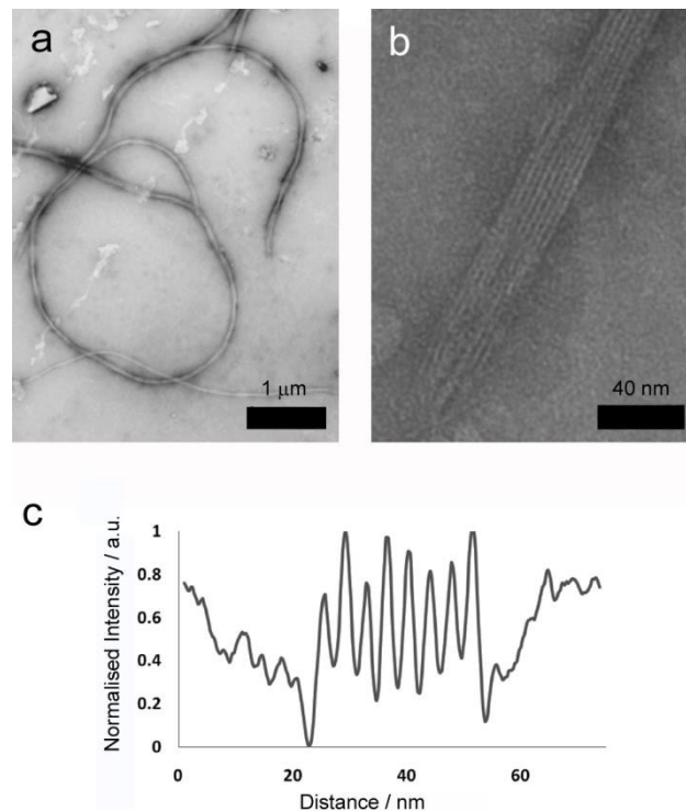
Figure 3. TEM images and analysis of a) long, flexible (scale bar 1\text{ }\mu\text{m} ) and b) striated fibres present in 20\text{ mM} total peptide hydrogel samples (scale bar 40\text{ nm} ). c) TEM intensity profile perpendicular to the long axis in a striated fibre with tape morphology.
