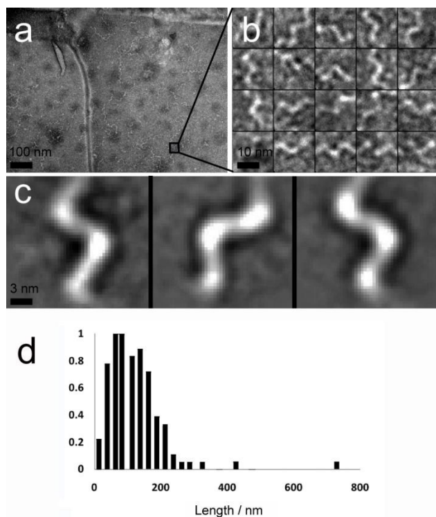
Figure 4: a) Contrast-enhanced TEM image showing numerous hydrogel fibrils with a twisted or helical appearance (scale bar 100 nm). b) TEM image of a selection of images of twists/helical repeats in hydrogel fibrils (scale bar 10 nm). c) Projection averages of selected images from b), demonstrating that these repeats are regular and consistent with a helical structure (scale bar 3 nm). d) Length distribution (normalised to highest frequency, 18, n = 118 ) of fibrils within 10 mM peptide hydrogel samples.
