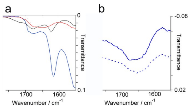
Figure 2. Selected regions from water subtracted ATR-FTIR spectra of: a) Standard p1 + p2 gel samples at pH 1 (—), 14 (—), and 7 (—). b) 10\text{ mM p1} at pH 7 (---); 10\text{ mM p2} at pH 7 (—).
