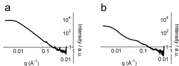
Figure 5: Porod analysis of SAXS profiles of: a) 5 mM p1 , pH 7.4, 20 °C and b) 5 mM p1 and 5 mM p2 , pH 7.4, 20 °C
