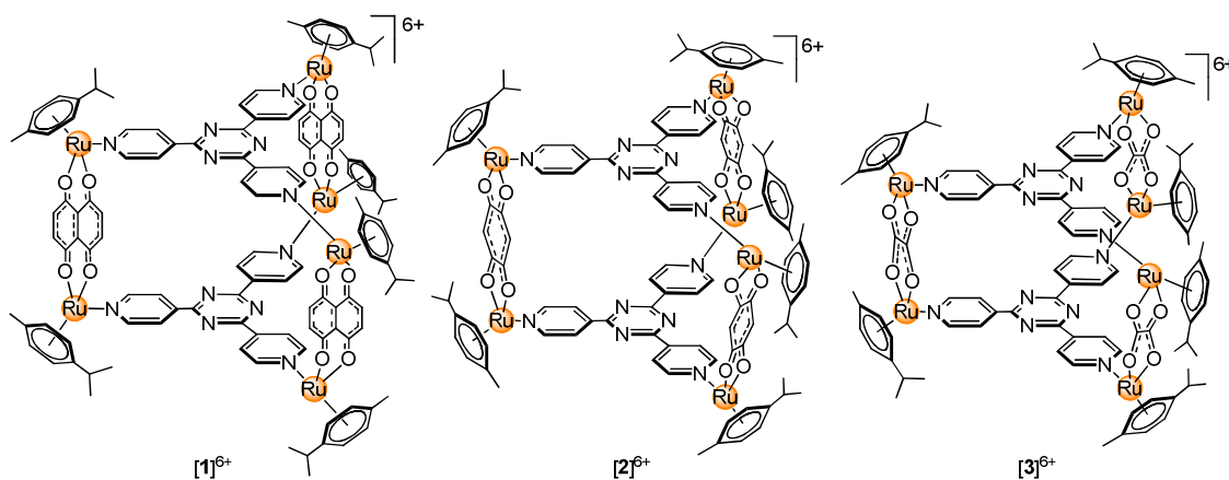
Figure 1. Structures of the hexacationic metallaprisms [1]^{6+} , [2]^{6+} and [3]^{6+} .
