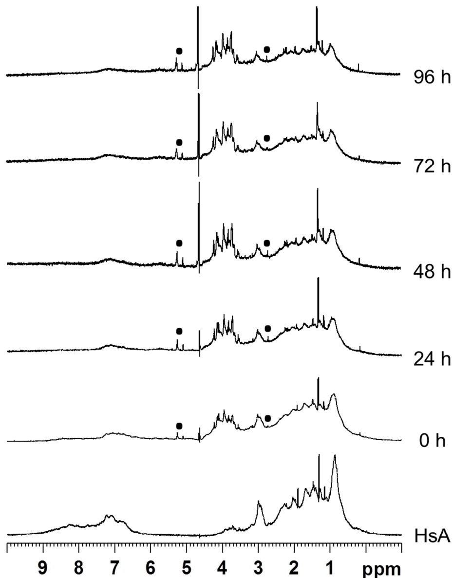
Figure 2. 1 H NMR spectra of the mixture HsA/[1] 6+ (molar ratio 1:10) recorded in D 2 O at 37 °C between 0 h and 96 h. The 1 H NMR spectrum of free HsA is shown at the bottom as reference. The p -cymene resonances of the metallaprism are labelled by (■).
