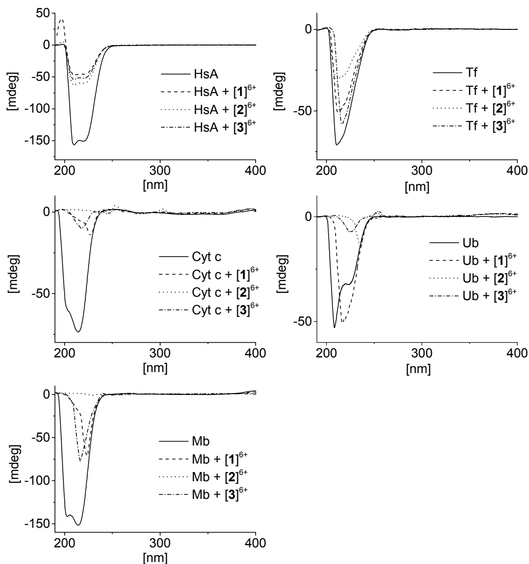
Figure 4. CD spectra of the mixtures containing the proteins and the metallaprisms (molar ratio 1:10). Left column: top = HsA, middle = Cyt c, bottom = Mb; right column: top = Tf, bottom = Ub.
