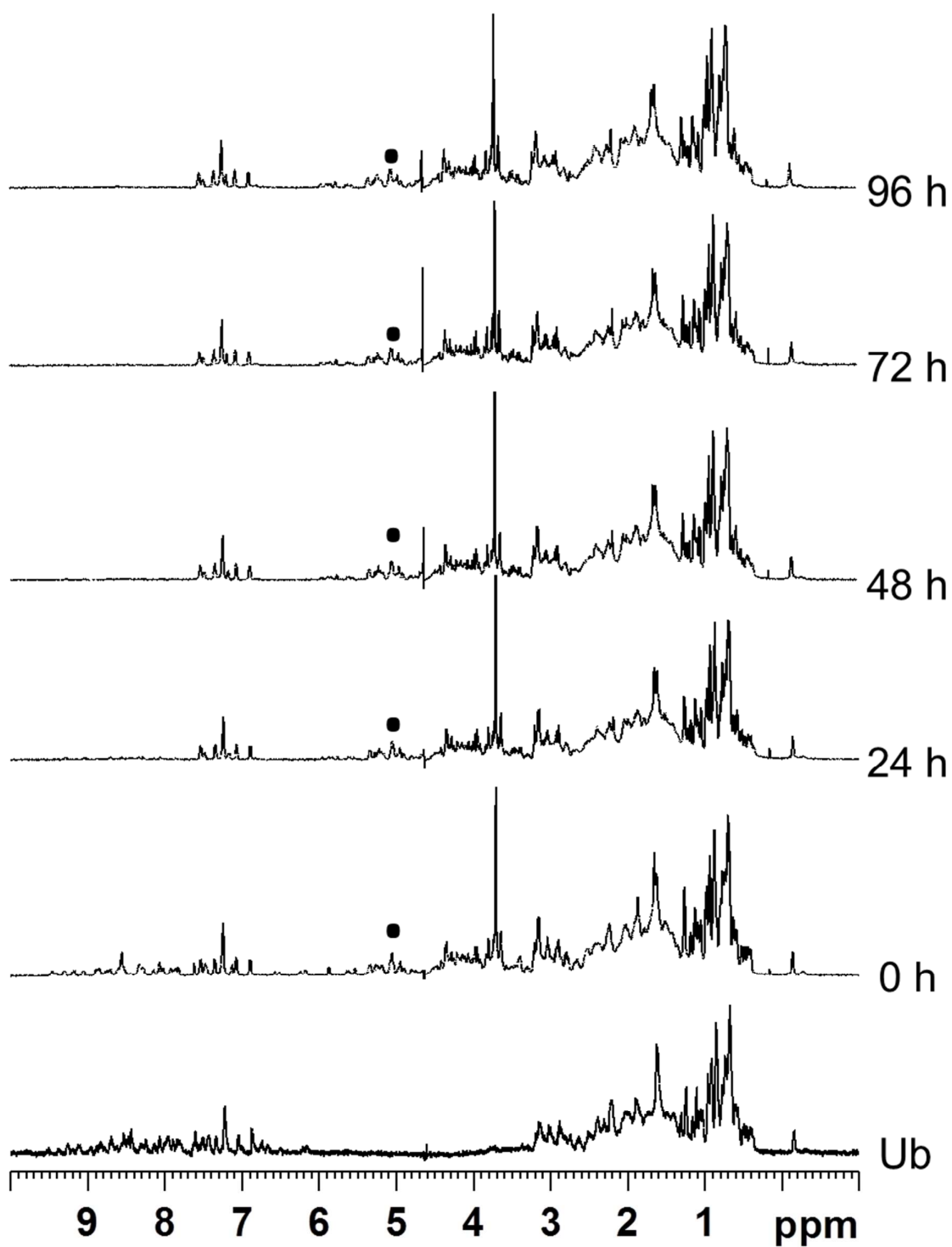
Figure 3. ^1\text{H} NMR spectra of the mixture Ub / [\mathbf{1}]^{6+} (molar ratio 1:10, \text{D}_2\text{O} , 37^\circ\text{C} ) recorded between 0 h and 96 h. The ^1\text{H} NMR spectrum of free ubiquitin is shown as reference at the bottom. The p -cymene resonances of the metallaprism are labelled by (■).
