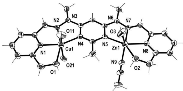
Figure 5. View of the [\text{CuZnL1}(\text{SO}_3\text{CF}_3)_2(\text{CH}_3\text{CN})(\text{H}_2\text{O})]^{2+} cation of complex 3 (crystallographic numbering). Thermal ellipsoids are drawn at the 50 % probability level (the \text{SO}_3\text{CF}_3^- anions coordinated to Cu1 have been simplified to O11 and O21 for clarity).
