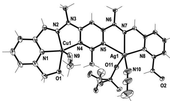
Figure 4. View of the [\text{CuAgL1}(\text{SO}_3\text{CF}_3)(\text{CH}_3\text{CN})_2]^{2+} cation of complex 2 (crystallographic numbering). Thermal ellipsoids are drawn at the 50 % probability level.
