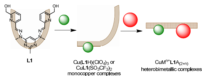
Figure 2. The two step, one pot synthetic strategy employed to form the heterobimetallic \text{CuM}^{n+}\text{L1A}_{(2+n)} complexes (where \text{M}^{n+} = \text{Pb}(\text{II}) , \text{Ag}(\text{I}) or \text{Zn}(\text{II}) , and \text{A} = \text{ClO}_4^- or \text{SO}_3\text{CF}_3^- ).
