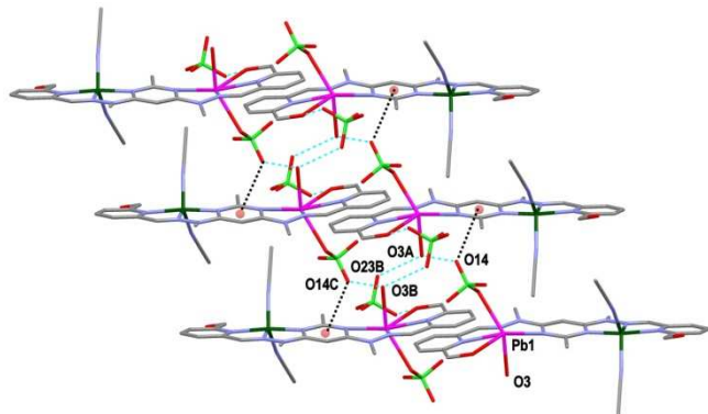
Figure 6. View of the arrangement of complex 1 into a one dimensional chain in the [1\ 0\ 0] direction through H-bonding. The anion- \pi interaction between O14 and the central pym rings is also shown (hydrogens have been omitted for clarity; symmetry codes A: -1+x, y, z ; B: -x, 1-y, -z ).
