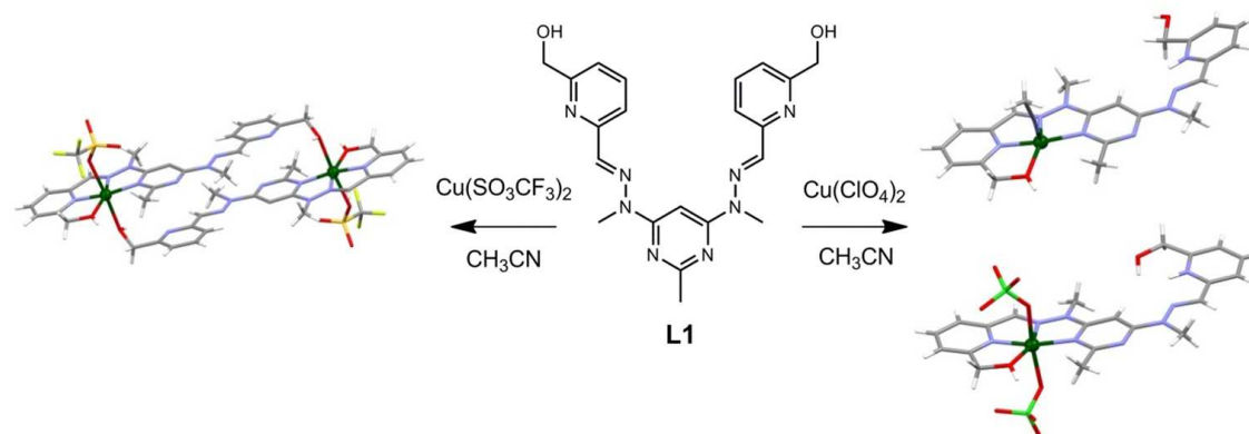
Figure 1. Solid state structures of the (right) \text{Cu}(\text{L1H})(\text{ClO}_4)_3 and (left) \text{CuL1}(\text{SO}_3\text{CF}_3)_2 complexes synthesised by reacting L1 with either \text{Cu}(\text{ClO}_4)_2 or \text{Cu}(\text{SO}_3\text{CF}_3)_2 in a 1:1 metal to ligand ratio. 8
