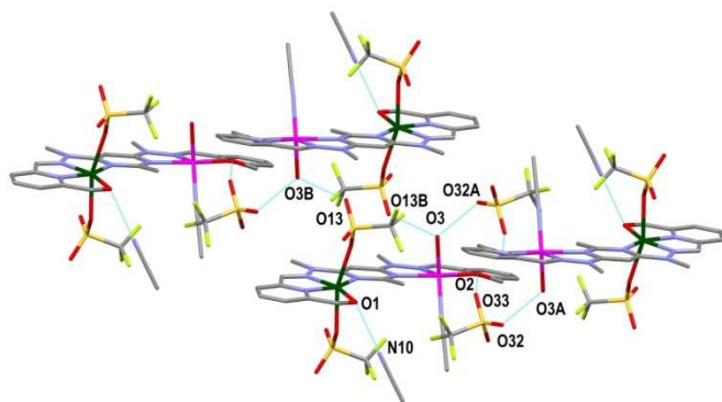
Figure 7. View of the arrangement of complex 3 into a one dimensional chain in the [1\ 0\ 0] direction through H-bonding. The H-bonding interaction between O1 and a \text{CH}_3\text{CN} molecule is also shown (hydrogens have been omitted for clarity; symmetry codes A: -x, -y, 1-z ; B: 1-x, -y, 1-z ).
