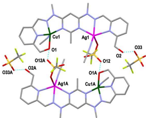
Figure 8. View of two [\text{CuAgL1}(\text{SO}_3\text{CF}_3)(\text{CH}_3\text{CN})_2]^{2+} cations of complex 2 joined as a dimer through H-bonding. Also shown
