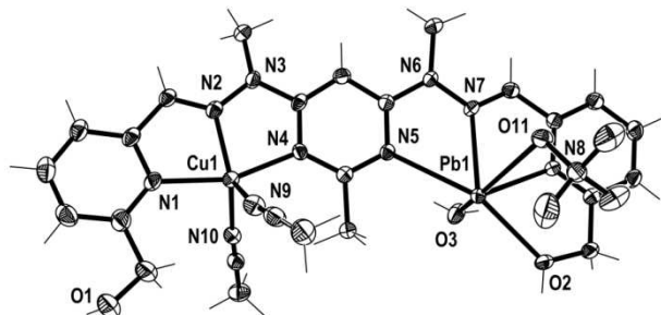
Figure 3. View of the [\text{CuPbL1}(\text{ClO}_4)(\text{CH}_3\text{CN})_2(\text{H}_2\text{O})]^{3+} cation of complex 1 (crystallographic numbering). Thermal ellipsoids are drawn at the 50 % probability level.
