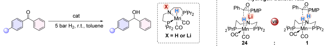
(B) Application of anionic catalysts in the hydrogenation
