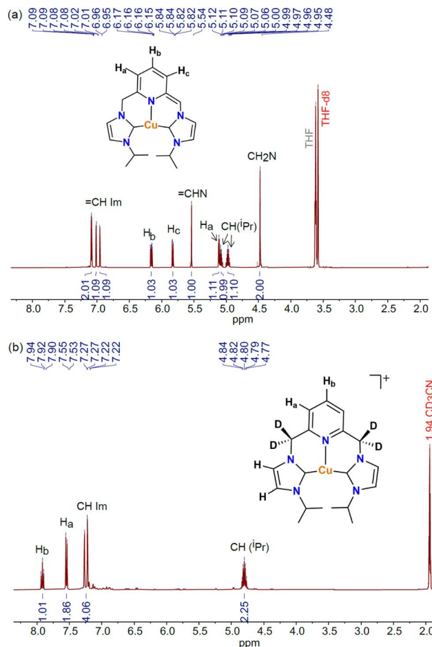
Fig. 4 (a) 1 H NMR spectrum (8.0–2.0 ppm) for [Cu( 1 Pr C N A C) * ], [Cu-L1 * ], in THF- d 8 at 298 K. (b) 1 H NMR spectrum (8.0–2.0 ppm) of the reaction of [Cu-L1]PF 6 (1 equiv.) and Cs 2 CO 3 (5 equiv.) in CD 3 CN after 24 h stirring at room temperature.
