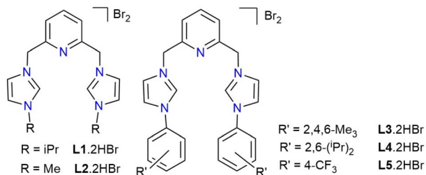
Fig. 1 The pincer \text{CNC}^R and \text{CNC}^{\text{Ar}} ligand precursors, R = i\text{Pr} (L1.2HBr), Me (L2.2HBr), Ar = Mes (L3.2HBr), Dipp (L4.2HBr), and p\text{-CF}_3\text{Ar} (L5.2HBr).
