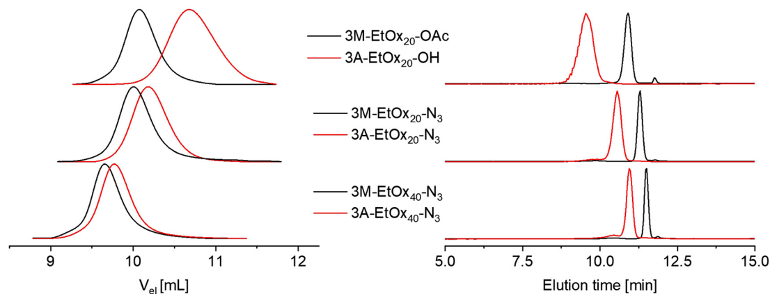
Fig. 6 Chromatographic analysis of protected and deprotected PETox heterotelechelic obtained by initiation of CROP with 3M. Left: SEC (RID). Right: HPLC (RP18 Chromolith column, water/acetonitrile gradient with 0.1% formic acid, ELSD).
