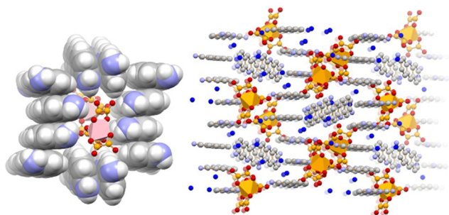
Fig. 7 \pi -Stacking of [HPF] + cations in crystalline [HPF] 3 [Ga(ox) 3 ] 2 ·4H 2 O (left), and encapsulation of two [Ga(ox) 3 ] 3- anions within a proflavinium-cation envelope (right). Reproduced from ref. 111.
