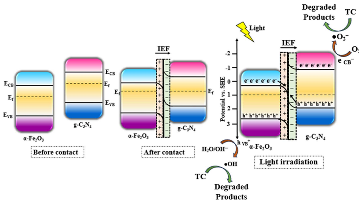
Scheme 3 Proposed S-scheme charge transfer mechanism in \alpha -Fe 2 O 3 /g-C 3 N 4 .
