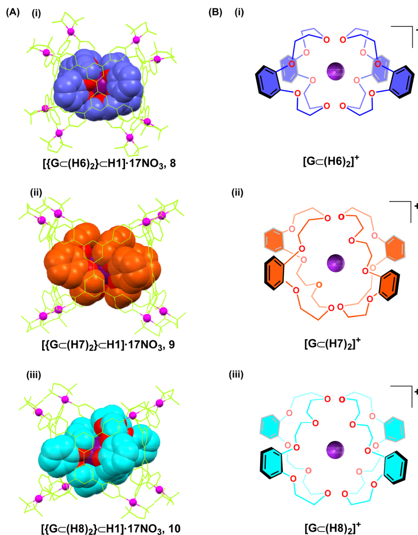
Fig. 8 (A) Crystal structures of 8 , 9 and 10 showing the super-host framework as a wireframe and the [\text{Cs}(\text{crown ether})_2]^+ as a space filling model. (B) Chemical drawings showing the relative orientation of the pair of encapsulated crown ether rings wrapped around \text{Cs}^+ , i.e., the [\text{Cs}(\text{crown ether})_2]^+ moieties as observed in the crystal structures of 8 , 9 and 10 .
