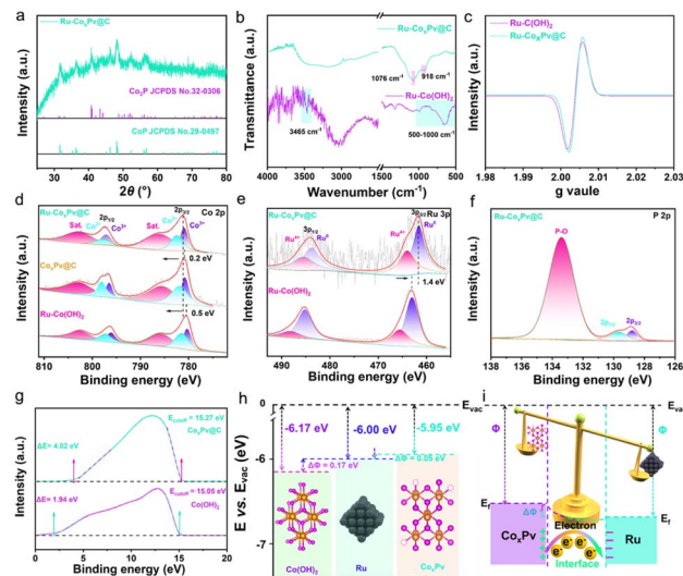
Fig. 2 (a) XRD pattern for \text{Ru-Co}_x\text{Pv@C} . (b) FT-IR spectra for \text{Ru-Co(OH)}_2 and \text{Ru-Co}_x\text{Pv@C} . (c) EPR spectra for \text{Ru-Co(OH)}_2 and \text{Ru-Co}_x\text{Pv@C} . (d) High-resolution Co 2p spectra for \text{Ru-Co(OH)}_2 , \text{Co}_x\text{P} and \text{Ru-Co}_x\text{Pv@C} . (e) Ru 3p XPS spectra for \text{Ru-Co(OH)}_2 and \text{Ru-Co}_x\text{Pv@C} and (f) P 2p XPS spectra for \text{Ru-Co}_x\text{Pv@C} . (g) UPS spectra for \text{Co(OH)}_2 , \text{Co}_x\text{Pv} and Ru. (h) Energy-band alignment diagram of \text{Co(OH)}_2 and \text{Co}_x\text{Pv} with respect to Ru. (i) Interfacial electronic configurations for HSo during the HER.
