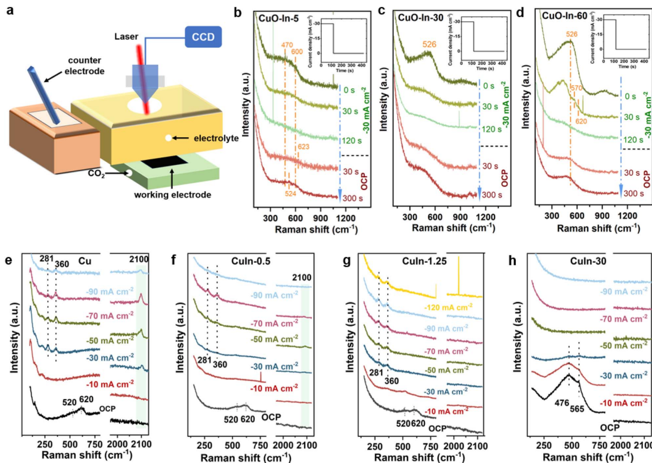
Fig. 4 In situ Raman spectra on Cu and CuIn catalysts. (a) Exploded view of the in situ Raman electrolysis flow cell. In situ Raman spectra and corresponding chronoamperograms (inset) of (b) CuO-In-5, (c) CuO-In-30 and (d) CuO-In-60 catalysts at -30 \text{ mA cm}^{-2} . In situ Raman spectra of the (e) Cu, (f) CuIn-0.5, (g) CuIn-1.25 and (h) CuIn-30 catalysts during electrochemical reduction of CO 2 at different current densities. CO 2 was continuously flowed to the cathodic gas chamber during measurement. A near-infrared laser (785 nm) was used as the excitation source. The spectra were collected at a range of 100–2200 cm -1 after sufficient electrolysis time to ensure the reduction of oxides. A representative spectrum of multiple measurements at steady state of the electrolysis is shown under each condition. Electrolyte: 0.5 M KHCO 3 . The spikes in some spectra are due to cosmic rays.
