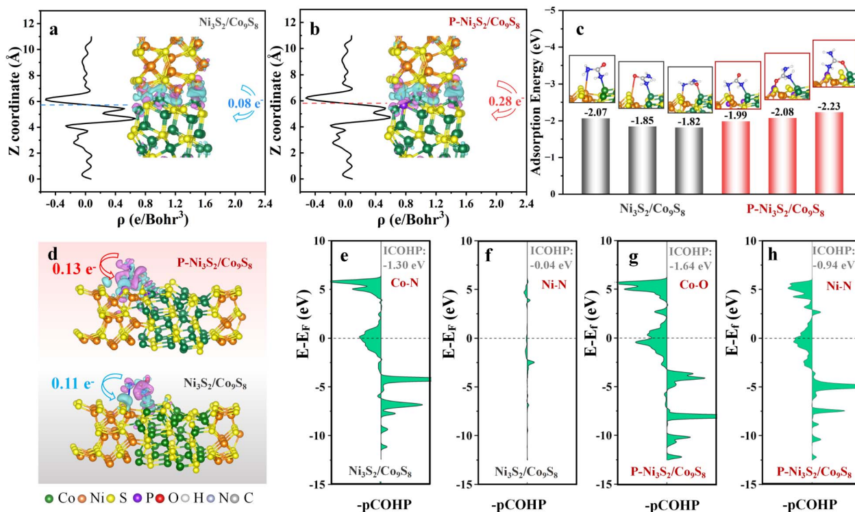
Fig. 5 Average charge density difference of (a) Ni_3S_2/Co_9S_8 and (b) P-Ni_3S_2/Co_9S_8 . (c) Three optimized adsorption structures and adsorption energies for CO(NH_2)_2 on Ni_3S_2/Co_9S_8 and P-Ni_3S_2/Co_9S_8 . (d) The difference charge density and Bader charge analysis for CO(NH_2)_2 on Ni_3S_2/Co_9S_8 and P-Ni_3S_2/Co_9S_8 , where the isosurface value is set to 0.0015\text{ e}^- \text{Å}^{-3} and the positive and negative charges are shown in cyan and magenta, respectively. The green, orange, yellow, purple, red, white, blue, and gray balls represent Co, Ni, S, P, O, H, N and C atoms, respectively. Projected crystal orbital Hamiltonian population (pCOHP) analysis between CO(NH_2)_2 and (e) and (f) Ni_3S_2/Co_9S_8 and (g) and (h) P-Ni_3S_2/Co_9S_8 .
