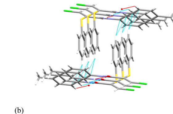
Fig. 5 Views, (a) and (b), from different angles showing the knitting of two chains of Z-3 together based on edge-to-face ( C-H\cdots\pi 2.83 Å) and face-to-face aromatic interactions.
