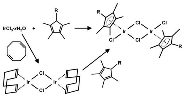
Scheme 1 Synthesis of the most used dinuclear intermediate, [\text{Ir}(\mu\text{-Cl})(\eta^5\text{-Cp}^x)\text{Cl}]_2 , for the synthesis of half-sandwich \text{Ir(III)} cyclopentadienyl complexes.
