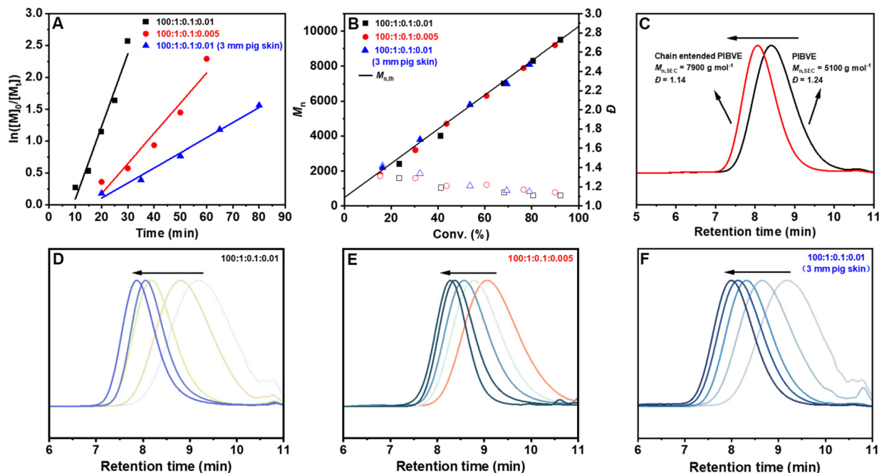
Fig. 2 Polymerization of IBVE with [\text{DPI}]_0/[\text{IR-780}]_0 = 0.1/0.01 , 0.1/0.005 and 0.1/0.01 (3 mm pig skin) under a 780 nm NIR light at 25 °C in toluene and DCM ( v/v = 9:1 ), V_{\text{IBVE}} = 1 mL, V_{\text{solvent}} = 1 mL. (A) \ln([M]_0/[M]_t) versus time. (B) Molecular weight ( M_n ) and molecular weight distribution ( D ) versus monomer conversion. (C) SEC traces of the PIBVE before and after chain extension. (D–F) SEC traces of the obtained PIBVE.
