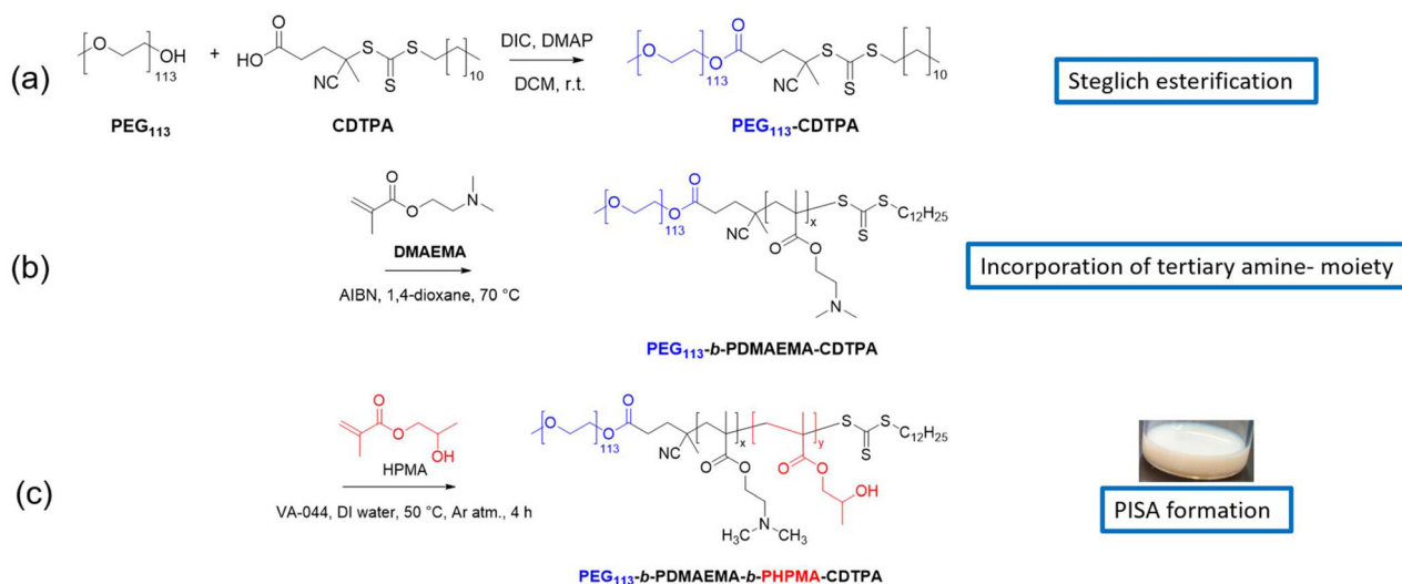
Scheme 1 (a) Synthesis of \text{PEG}_{113} -CDTPA via Steglich esterification. (b) Synthesis of \text{PEG}_{113} - b -PDMAEMA-CDTPA to incorporate the tertiary amine moiety responsible for anchoring MNPs. (c) Synthesis of \text{PEG}_{113} - b -PDMAEMA- b -PHPMA-CDTPA triblock copolymers via thermal RAFT-PISA to form milky stable suspensions.
