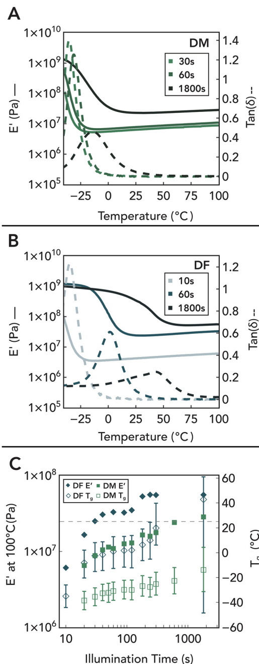
Fig. 8 (A) DMA traces of DM network polymers illuminated for 30 s, 60 s, and 1800 s. (B) DMA traces of DF network polymers illuminated for 10 s, 60 s, and 1800 s. (C) E' at 100^\circ\text{C} and T_g of DF and DM with error bars representing full width at half maximum of the glass transition. Collectively, these results suggest an increase in crosslinking density and network heterogeneity with continued light exposure.
