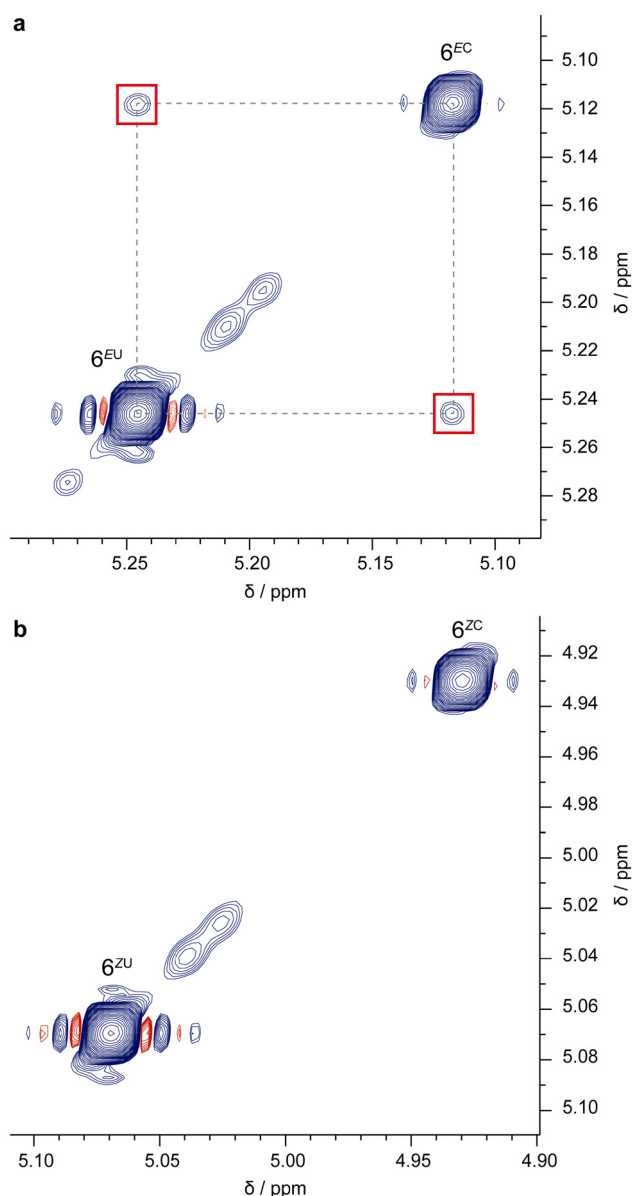
Fig. 5 Partial EXSY NMR ( CD_3CN , 500 MHz, 298 K, 1.4 mM, t_{mix} = 600 ms) spectra of (a) an equimolar mixture of EE\text{-}4H^+ and 2 , and (b) the same sample after exhaustive irradiation at 365 nm. 6^{EU} and 6^{EC} in (a) indicates the free and complexed EE axle, respectively, whereas 6^{ZU} and 6^{ZC} in (b) denote the free and complexed ZZ axle, respectively.
