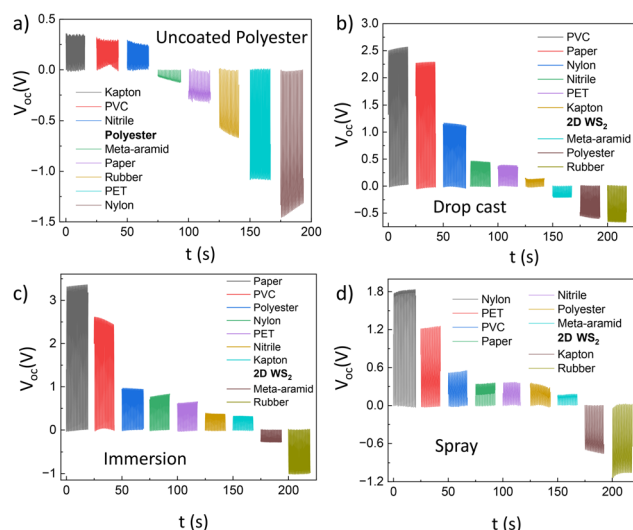
Fig. 3 Triboelectric series based on open-circuit voltage measurements over time for different triboelectric layers of TENGs tested with (a) uncoated polyester, (b) polyester coated with 2D WS 2 via drop casting, (c) polyester coated with 2D WS 2 via immersion, and (d) polyester coated with 2D WS 2 via spray.
