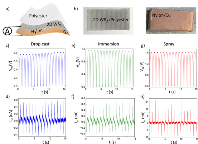
Fig. 2 (a) Schematic of the flexible textile-based triboelectric nanogenerator, working in a single-electrode configuration, fabricated using 2D WS 2 coated onto the polyester fabric as a triboelectric layer, with nylon serving as the counter triboelectric pair and copper acting (Cu) as an electrode. (b) Photographs of the parts of the TENG device with an area of 1.5\text{ cm} \times 2.5\text{ cm} . Open-circuit voltage ( V_{oc} ) and short-circuit current ( I_{sc} ) vs. time for 2D WS 2 coated via drop casting (c) and (d), respectively. V_{oc} and I_{sc} for 2D WS 2 coated via immersion (e) and (f), respectively. V_{oc} and I_{sc} for 2D WS 2 coated via spray (g) and (h), respectively.
