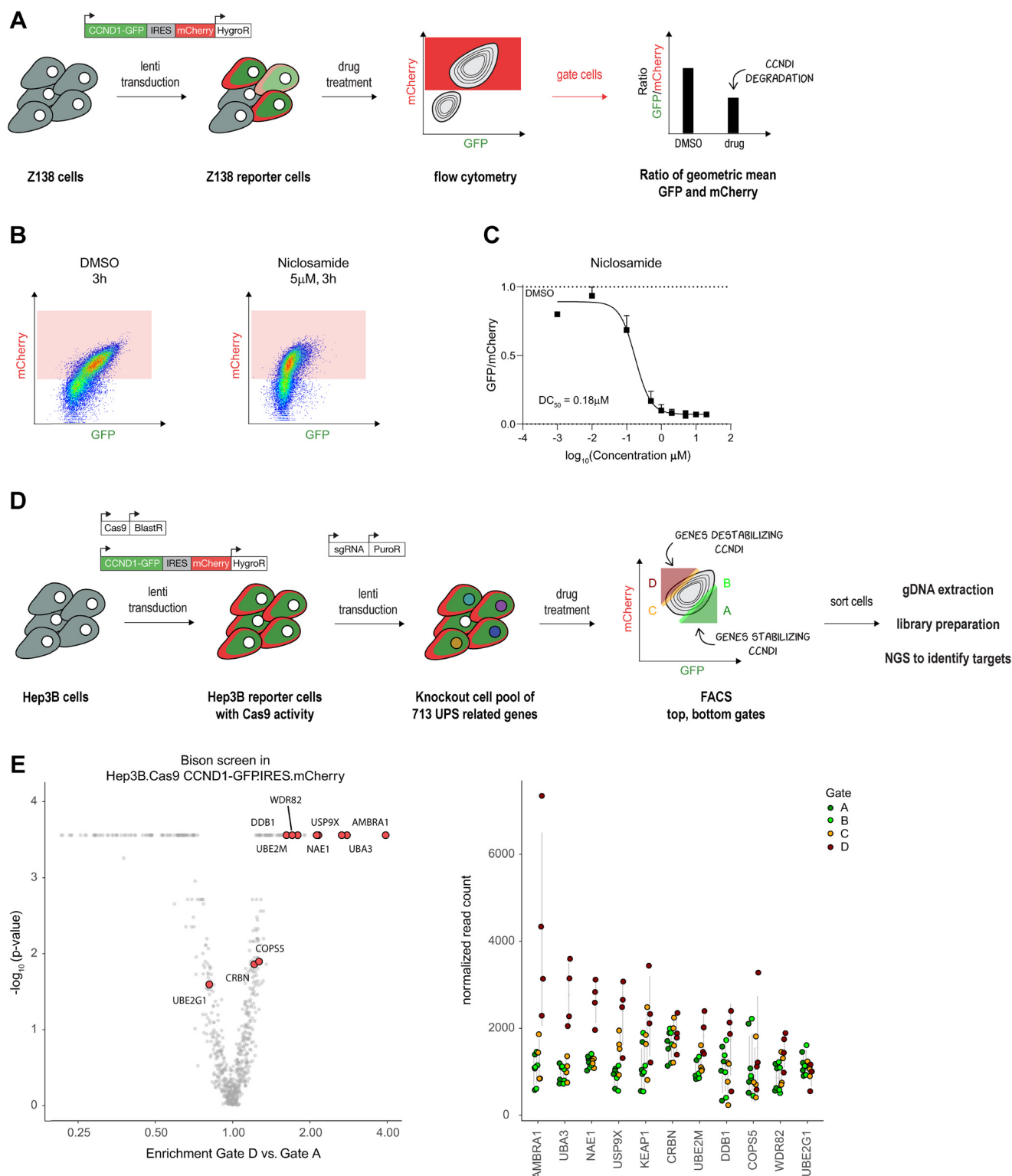
Fig. 2 CCND1 reporter cell lines capture degradation activity. A ) Set-up towards establishing the fluorescence-based reporter system for quantifying CCND1 protein levels in Z138 cells. B ) The population of Z138 reporter cells (Z138 CCND1-GFP.IRES.mCherry) gated by flow cytometry and used for quantification of CCND1. C ) Dose response curve of CCND1 levels relative to vehicle (DMSO) treatment in the reporter cells treated with niclosamide for 3 h. Values represent the ratio of the geometric mean of GFP and mCherry values in the gated population. D ) Workflow of setting up a CCND1 reporter in Hep3B cell with Cas9 activity and performing a FACS based genetic screen of members of the UPS which can rescue drug induced CCND1 degradation. E ) Genes enriched in a FACS based genetic CRISPR screen (Bison library) rescuing niclosamide induced CCND1 degradation in Hep3B.Cas9.CCND1-GFP.IRES.mCherry reporter cells. The gates used are shown in D ) and each contain 5% of the population shown. Gate D contains cells with gene KO that stabilize CCND1, whereas gate A contains cells with gene KO that destabilize CCND1.
