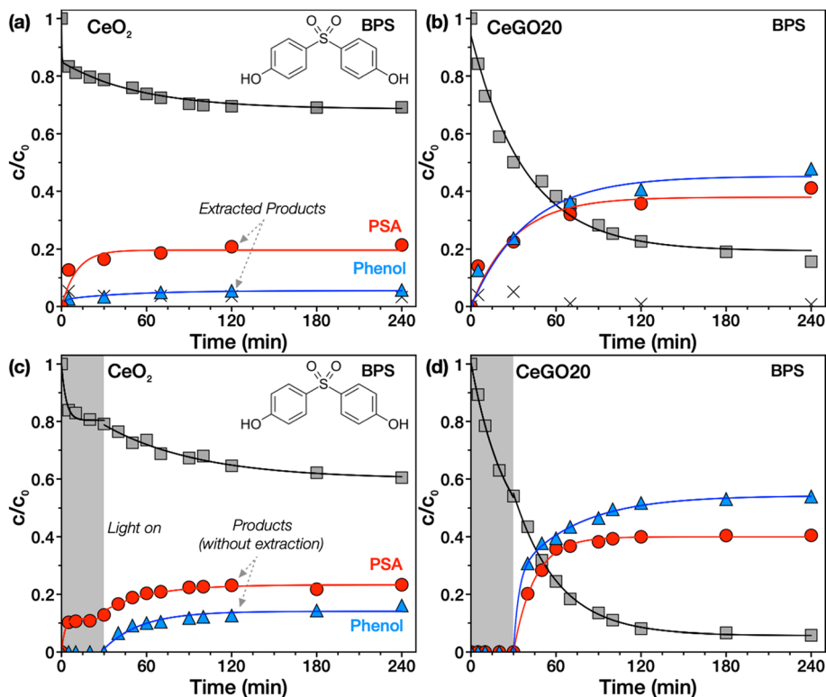
Fig. 6 Reactive adsorption of BPS on (a) CeO 2 and (b) CeO 2 nanoparticles grown on GO (representative sample CeGO 20 ); solar-light enhanced photodecomposition of BPS on (c) CeO 2 and (d) sample CeGO 20 . Color coding: black squares – BPS concentration in solution, black crosses – BPS extracted from the surface of the catalyst, red circles – PSA and blue triangles – phenol (both extracted in the case of dark tests or released and analyzed directly in solution in photocatalytic tests).
