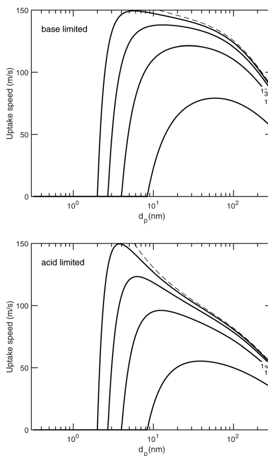
Fig. 17 Uptake speed ( \gamma_{i,p} S_{i,p}^{\text{flat}} , black curves) vs. the diameter for flat-surface saturation ratios S^{\circ} = \{3, 10, 30, 100\} and d_{\text{K}10} = 2 \text{ nm} . The S^{\circ} = \infty limit is shown as a dashed curve. (Top) Base-limited ( \text{NH}_3 ) limited uptake assuming no van der Waals enhancement ( A = 0 joule). (Bottom) Acid-limited ( \text{HONO}_2 ) uptake with significant van der Waals enhancement ( A = 6 \times 10^{-20} joule). The collision speed (and thus growth rates) increases rapidly after activation, reaches a maximum and then declines again. The maximum is especially sharp when the van der Waals enhancement is large ( i.e. for acid limited conditions in the lower panel).
