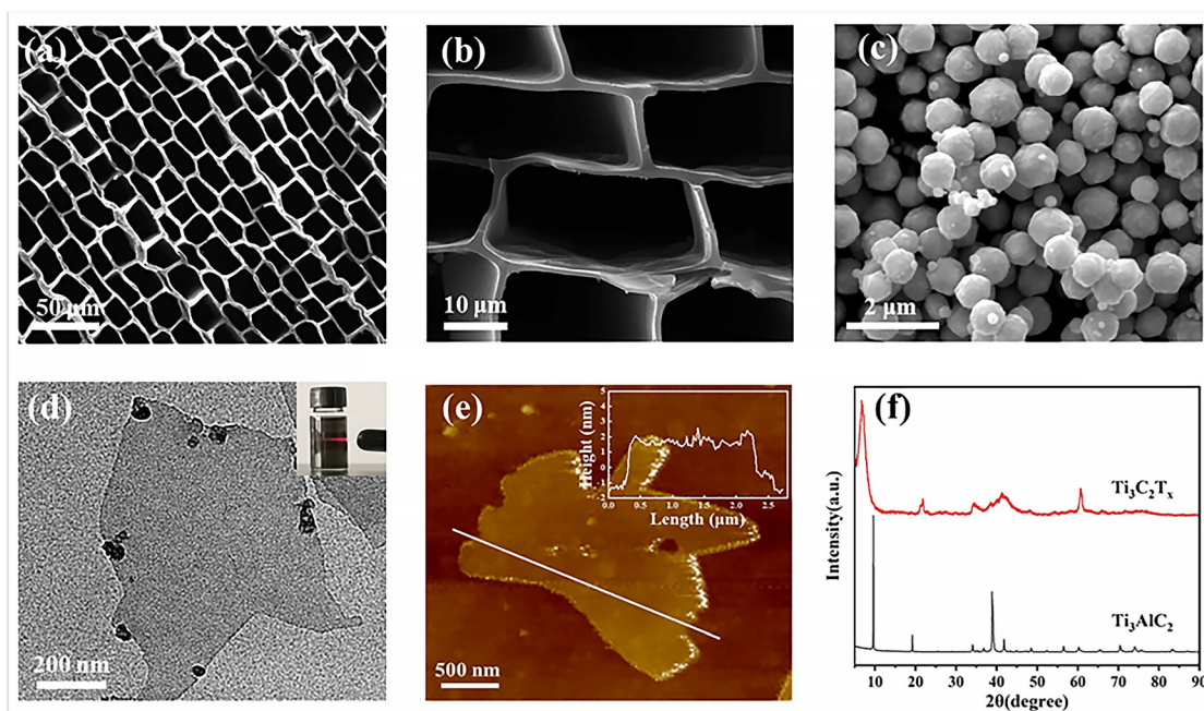
Fig. 2 SEM images of (a) cross-sectional wood, (b) high-magnification cross-sectional wood, and (c) CoNi. (d) TEM image of Ti 3 C 2 T x MXene. (e) AFM image of Ti 3 C 2 T x MXene. (f) XRD patterns of Ti 3 AlC 2 and Ti 3 C 2 T x MXene.
