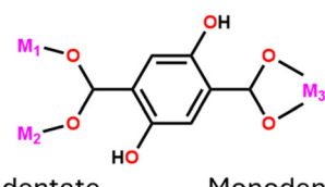
Fig. 4 Scheme of the bidentate and monodentate coordination modes of the DOBDC linker.
