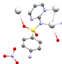
Fig. 3 Crystal structure of the new \text{AgSD-NO}_3 (colour code: red – oxygen; blue – nitrogen; grey – carbon; yellow – sulfur; light grey – silver).
