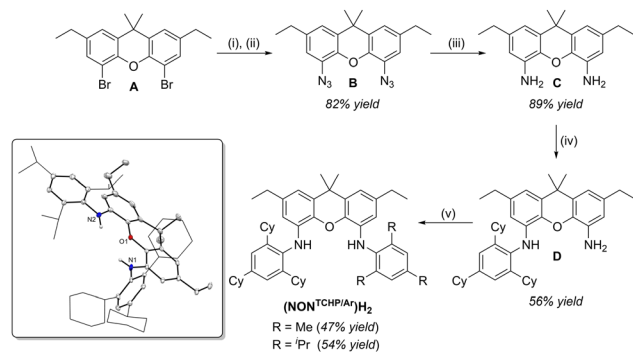
Scheme 1 Synthesis of unsymmetrical bis(anilino)xanthene pro-ligands. (i) n\text{BuLi} (2 equiv.), THF, -78^\circ\text{C} . (ii) Tosylazide (2 equiv.), THF, -78^\circ\text{C} – RT, 18 h. (iii) \text{LiAlH}_4 (3 equiv.), \text{Et}_2\text{O} , reflux, 2 h. (iv) (\text{TCHP})\text{Br} (1 equiv.), \text{Pd}(\text{OAc})_2 (4 mol%), \text{DPEPhos} (6 mol%), \text{NaOtBu} (1.4 equiv.). (v) (\text{Mes})\text{Br} (1 equiv.) or (\text{Trip})\text{Br} (1 equiv.), \text{Pd}(\text{OAc})_2 (4 mol%), \text{DPEPhos} (6 mol%), \text{NaOtBu} (1.4 equiv.). Inset: Molecular structure of (\text{NON}^{\text{TCHP}/\text{Trip}})_2 . Thermal ellipsoids shown at 15% probability; hydrogen atoms (except amine protons) omitted; cyclohexyl and isopropyl groups shown in wireframe for clarity.
