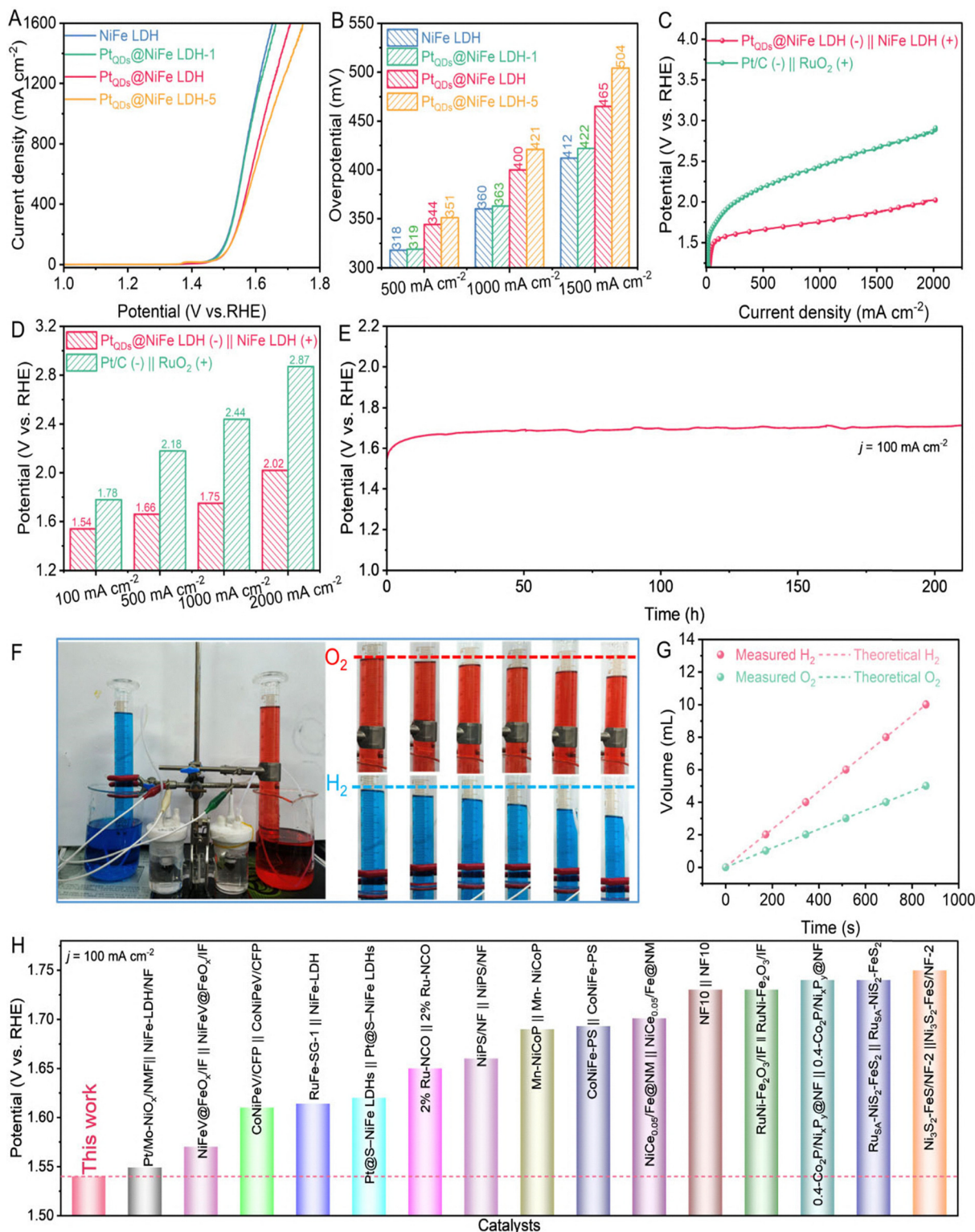
Fig. 11 OWS results; (A) LSV plots; (B) plot depicting comparison of overpotentials at different current densities; (C) potential vs. current density plots Pt OD5 @NiFe LDH (-)||NiFe LDH (+) and Pt/C (-)||RuO 2 ; (D) plot of potential (cell voltage) vs. current density (E) potential vs. time plot depicting stability in OWS process; (F) snapshots representing the OWS experimental set up and extent of gas collection at different instances; (G) plot depicting measured volume of H 2 or O 2 against theoretically produced H 2 or O 2 w.r.t. time; (H) potential comparison of Pt OD5 @NiFe LDH (-)||NiFe LDH (+) over other reported electrocatalysts (reproduced with permission from ref. 61©OAE publishing, Inc.; License: CC-BY 4.0).
