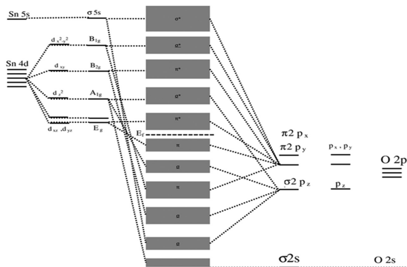
Fig. 8 Molecular-orbital bonding structure for tetragonal \text{SnO}_2 .
