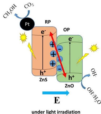
Fig. 11 Diagrammatic representation of the S-scheme mechanism of the photogenerated charge carrier transfer process, where \vec{E} denotes the electric field's direction. Drawn from scholarly sources (Mohamed et al. , 2021).
