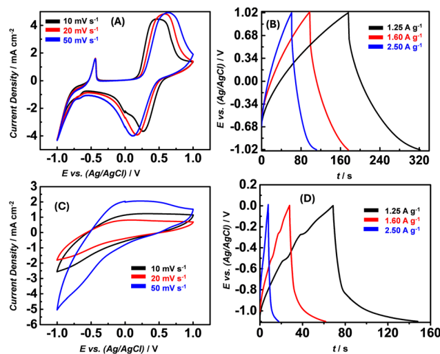
Fig. 4 Electrochemical performances of flavin-based electrodes in the PEO-KOH gel electrolyte in three-electrode systems. (A) Cyclic voltammograms at different scan rates from 10 to 50 mV s −1 for cFI . (B) GCD curves at different current densities from 1.25 to 2.5 A g −1 for cFI . (C) Cyclic voltammograms at different scan rates from 10 to 50 mV s −1 for FI and (D) GCD curves at different current densities from 1.25 to 2.5 A g −1 for FI .
