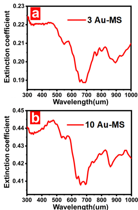
Fig. 5 Extinction spectra of (a) the triangle structure with 3 Au microspheres and (b) the pagoda-like microcavity with 10 Au microspheres.
