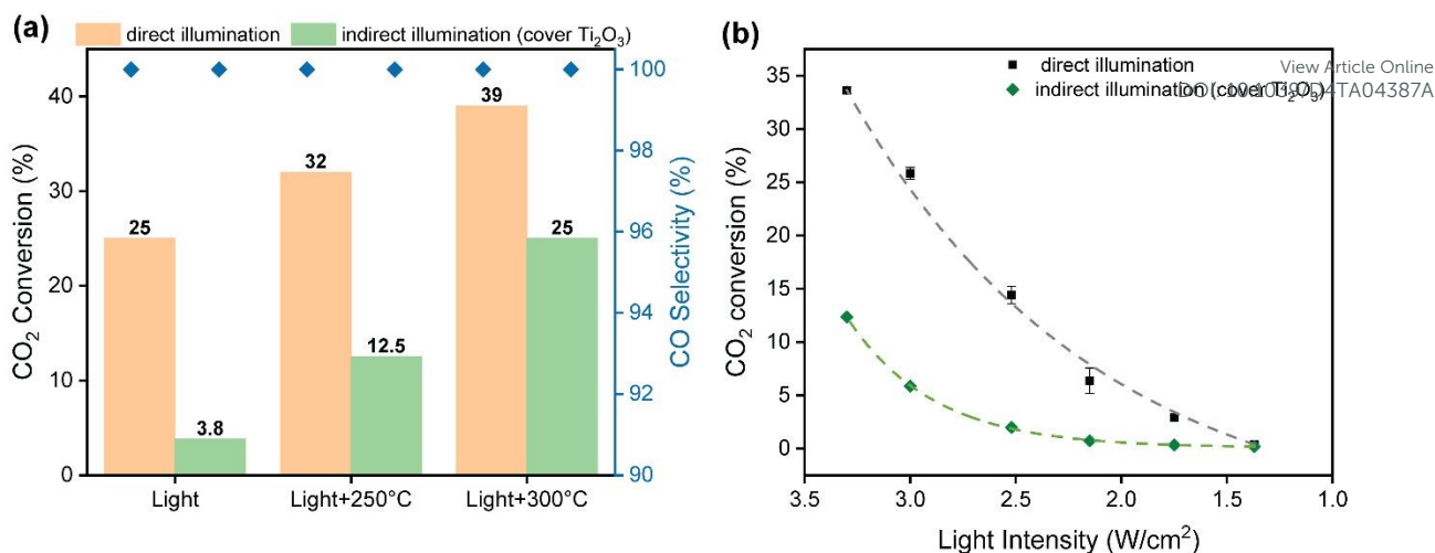
Fig. 3 a) CO 2 conversion and CO selectivity over Cs-promoted In 2 O 3 under direct and indirect illumination of 3.3 W·cm -2 without and with external heating. Reaction conditions: GSHV = 15000 mL·h -1 ·g -1 , 1 bar. b) Study of the effect of light intensity on the CO 2 conversion over Cs-promoted In 2 O 3 catalyst under direct and indirect illumination. Reaction conditions: GSHV = 15000 mL·h -1 ·g -1 , 1 bar, 250 °C.
