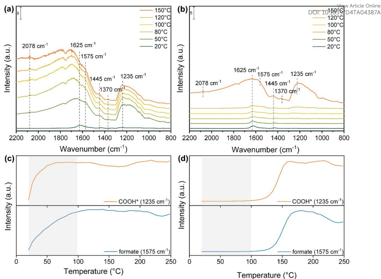
Fig. 4 In-situ DRIFTS spectra of Cs-promoted \text{In}_2\text{O}_3 under \text{H}_2 and \text{CO}_2 (4:1) at 10 bar with increased temperature upon a) light and b) dark conditions. IR peak intensities of \text{COOH}^* and bidentate formate species as a function of temperature under c) light and d) dark conditions.
