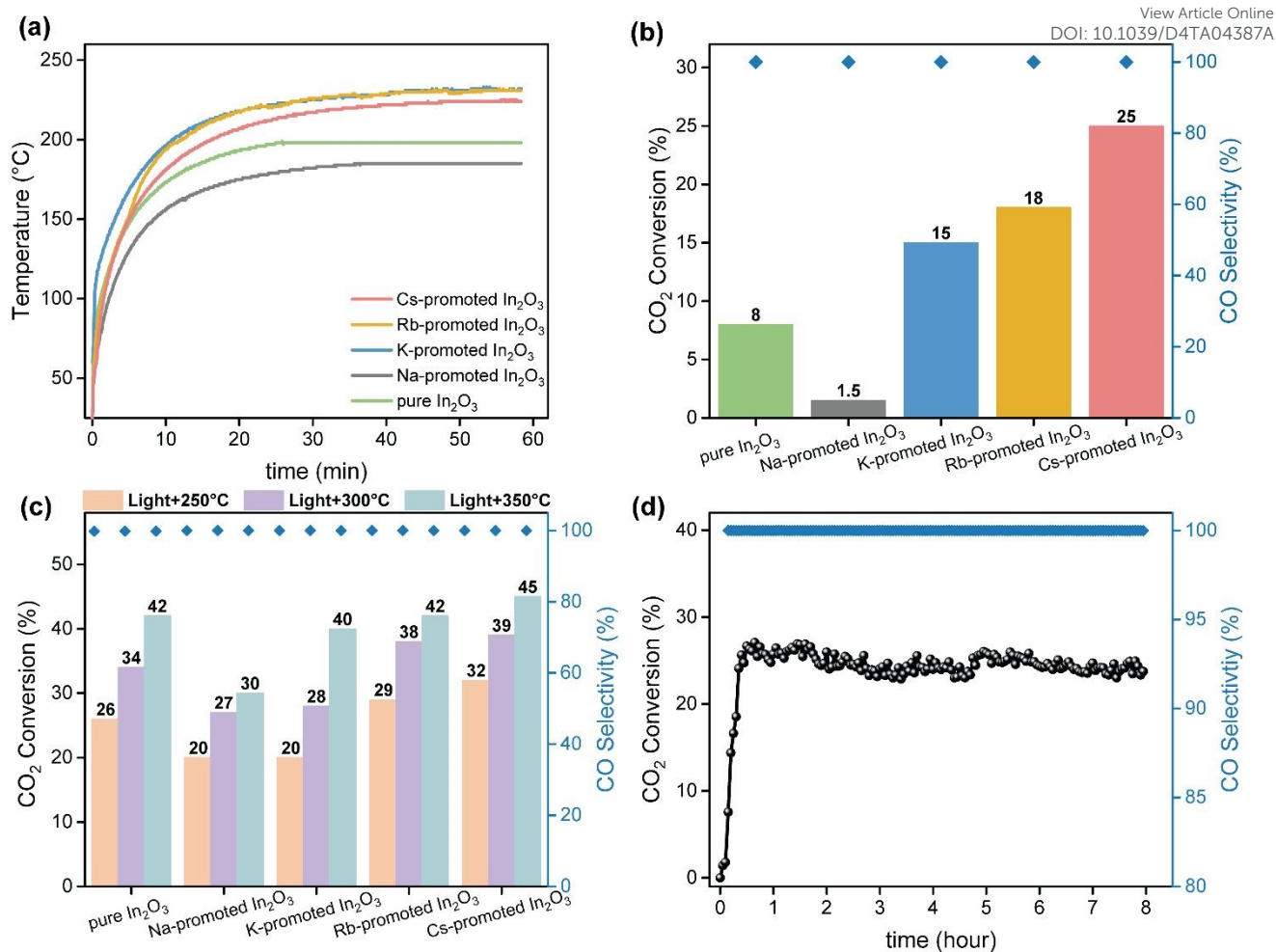
Fig. 2 a) Temperature evolution over pure and alkali-promoted catalysts under 3.3 W·cm -2 light irradiation. b) CO 2 conversion and CO selectivity over pure and alkali-promoted In 2 O 3 without external heating under irradiation of 3.3 W·cm -2 . Reaction conditions: GSHV = 15000 mL·h -1 ·g -1 , 1 bar. c) CO 2 conversion and CO selectivity over pure and alkali promoted In 2 O 3 with external heating at 250, 300 and 350 °C under irradiation of 3.3 W·cm -2 . Reaction conditions: GSHV = 15000 mL·h -1 ·g -1 , 1 bar. d) Stability test of Cs-promoted In 2 O 3 with external heating at 250 °C under irradiation of 3 W·cm -2 . Reaction conditions: GSHV = 15000 mL·h -1 ·g -1 , 1 bar.
