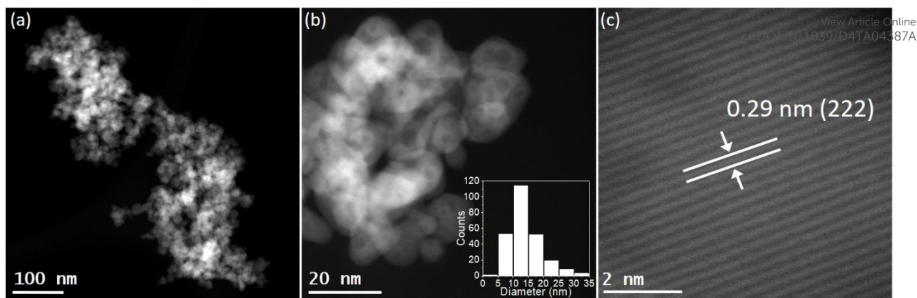
Fig. 1 STEM images of Cs-promoted \text{In}_2\text{O}_3 at a) low and b) high magnification. Inset in b) corresponds to the particle size distribution. c) Interplanar distance corresponding to the lattice distance of (222) plane of \text{In}_2\text{O}_3 .
