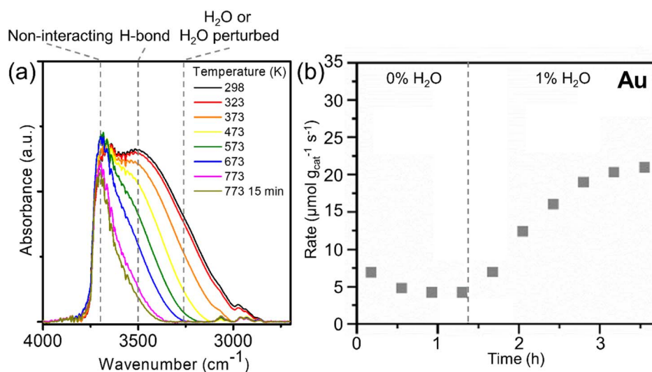
Fig. 1 (a) In situ FTIR spectra of as-prepared Au RCT-SiO 2 in the 4000–2700 cm -1 region collected as a function of temperature from 298 to 773 K in \text{O}_2 . (b) The rate of 1-propanol oxidation over Au RCT-SiO 2 in the absence and presence of co-fed 1% \text{H}_2\text{O} at 423 K. Dashed lines in (a) denoted the assignments of silanol groups. Reaction conditions in (a): 100% \text{O}_2 ; flow rate = 20 \text{ mL min}^{-1} , (b): 4% 1-propanol, 10% \text{O}_2 , 0 or 1% \text{H}_2\text{O} , balanced in He; total flow rate = 50 \text{ mL min}^{-1} ; m_{\text{cat}} = 10.0 \text{ mg} .
